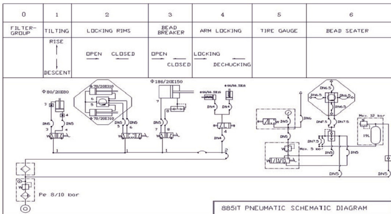
Pneumatic schema
