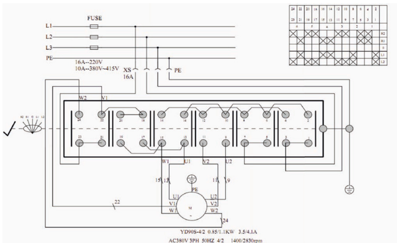
Electrical schema
